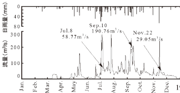
図-2 雨量と流量の関係 Fig. 2 Relationship between rainfall and runoff
